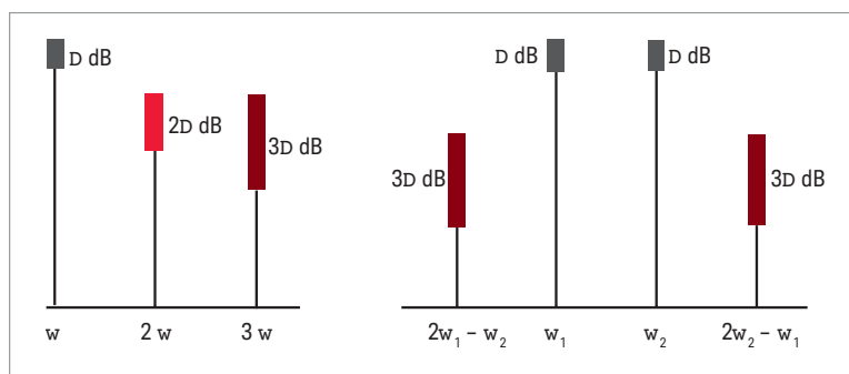
Figure 6-1. Changing the level of fundamental tones at the mixer
