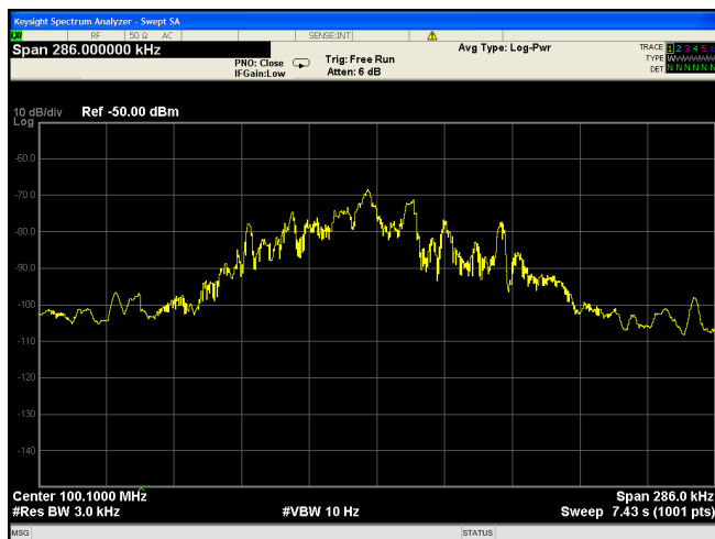
Figure 2-32a. Video filtering
