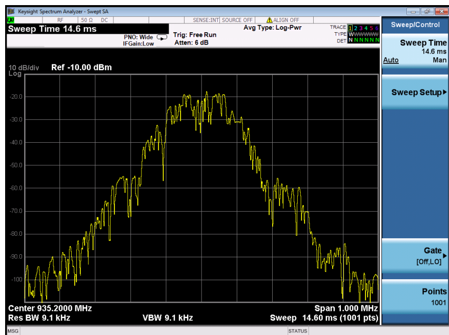
Figure 2-41. Spectrum of the GSM signal
