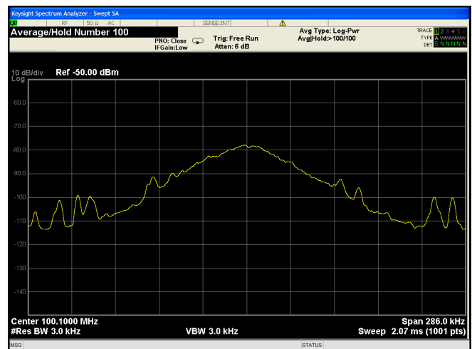
Figure 2-32b. Trace averaging
