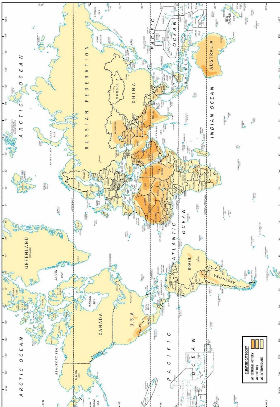
Figure C-1. Areas of occurrence of climatic categories A1, A2, & A3.
