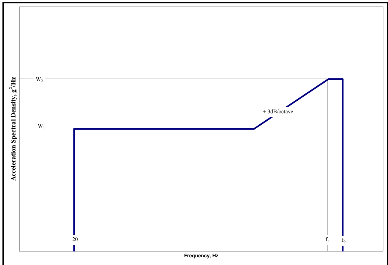
Figure 514.6D-5. Category 15 - Jet aircraft store vibration response.
